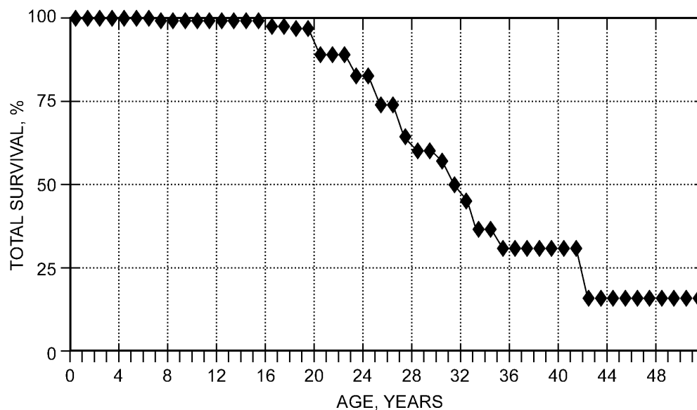
Fig. 1 Survival Curve for Centrifugal Chillers (Based on data from Abramson et al. 2005)
